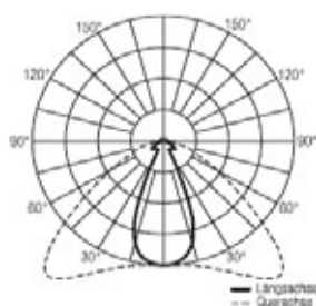
Light distribution 30°
