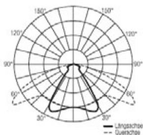
Light distribution 60°
