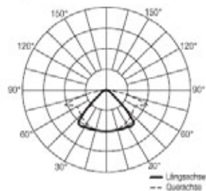
Light distribution 90°
